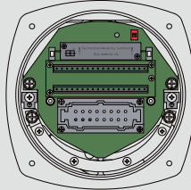
Plug-in terminals
